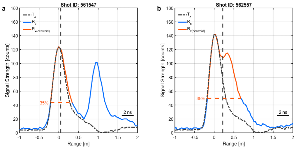
Figure 5. Example of complex return waveforms (blue) over a sea-ice pressure ridge. The transmit waveform is shown in dashed gray and scaled to the maximum amplitude of the return pulse to show the deviation of the return pulse. Multiple separate return pulses can be identified by the .count parameter (a), while return pulses much broader than the transmit pulse (b) will be revealed by larger values in the .width field. The vertical dashed line in both panels marks the location of the centroid, indicating that the centroid estimates from complex return pulses need to be interpreted properly.
