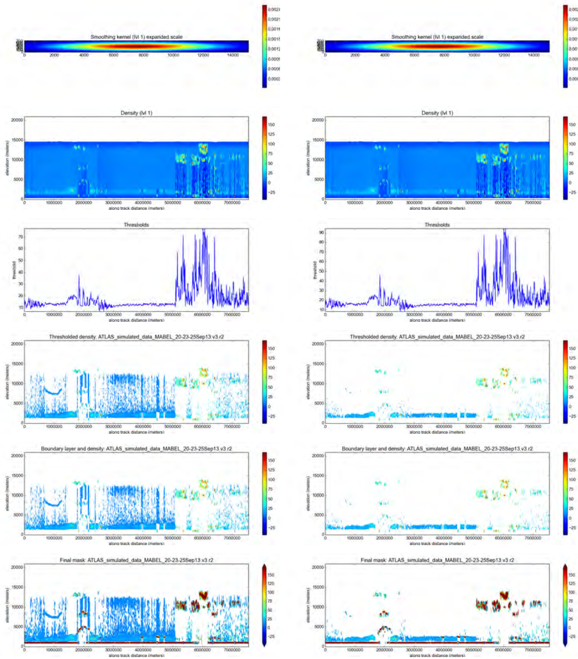
a) threshold_sensitivity = .9
