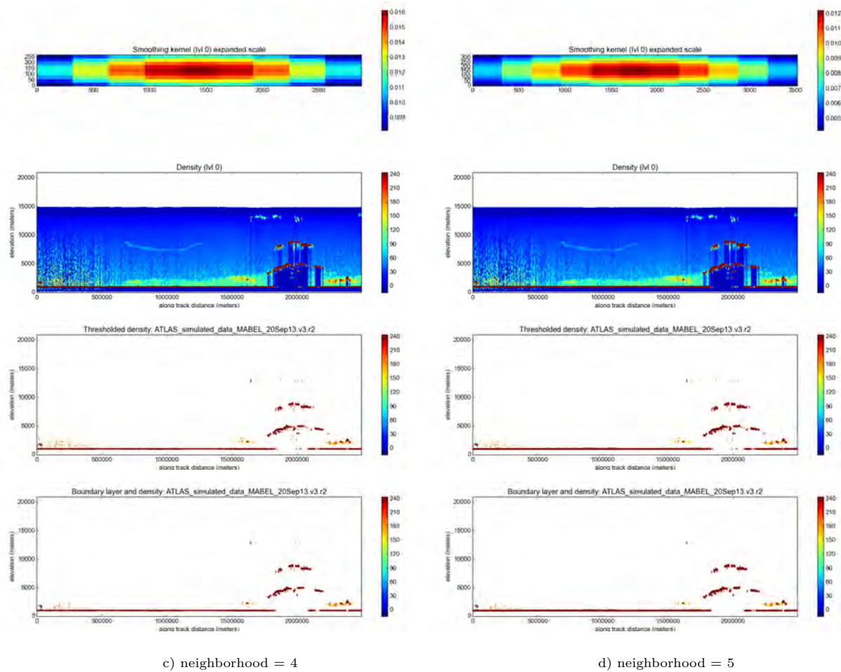
c) neighborhood = 4
