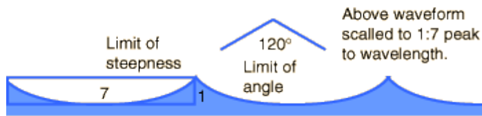
Figure 5. Trochoidal shape of surface waves at the limit of steepness, wavelength equal to seven times height. The sharply peaked trochoidal shape is common to all surface waves longer than capillary waves, which have an inverted trochoidal shape. At the steepness limit the waves begin to break. (Figure from http://hyperphysics.phy-astr.gsu.edu/hbase/waves/watwav2.html )
