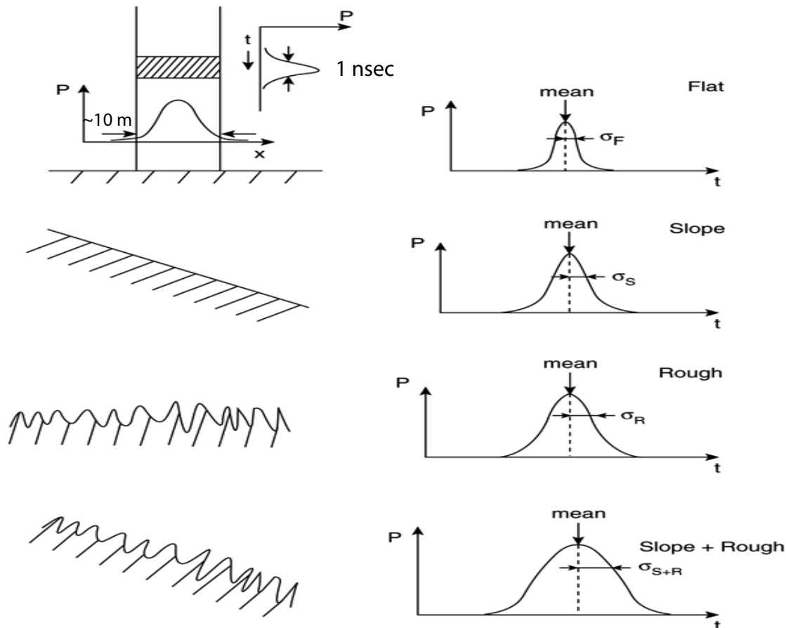
Figure 1. Characteristics of an idealized distribution of ATLAS return photon arrival times assuming a Gaussian instrument impulse response and a reflective surface with Gaussian roughness. In general surface slope and roughness both broaden the return distribution. For the open ocean the slope effect is likely negligible compared the effect of roughness due to surface waves. An important complication is that surface waves produce a non-Gaussian surface due to their broad troughs and narrow peaks.
