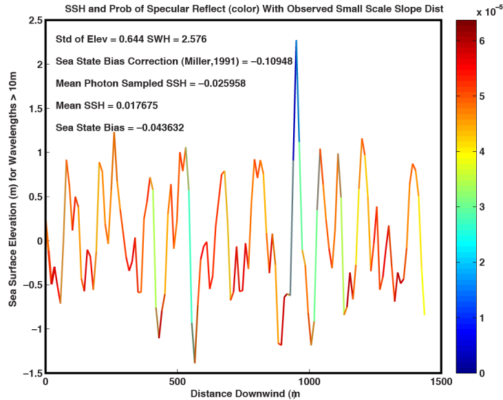
Figure 9. Height due to long-waves versus distance downstream (from upper right corner to lower left in Figure 6-left) with color-coded probability of specular reflection.
